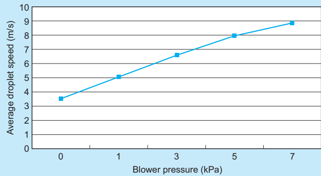
At distances under 150 mm, droplet speed is roughly proportional to blower pressure.
