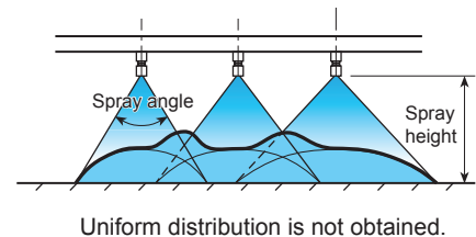
(A) Spray distribution of nozzles with no quality guarantee
