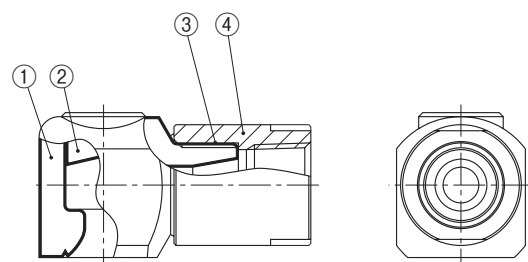
①Nozzle body ②Plate ③Adhesive: Araldite®H ④Socket (S316)
