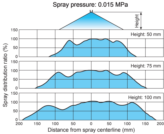
Relation between spray height and spray distribution
