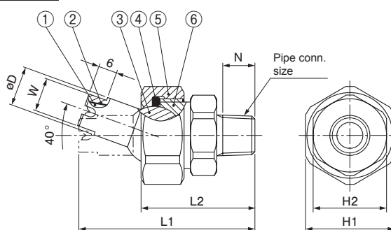
Nozzle tip (①Ceramic orifice ②Adhesive: Araldite® ③Ball) (④O-ring (NBR) ⑤Cap ⑥Adaptor
