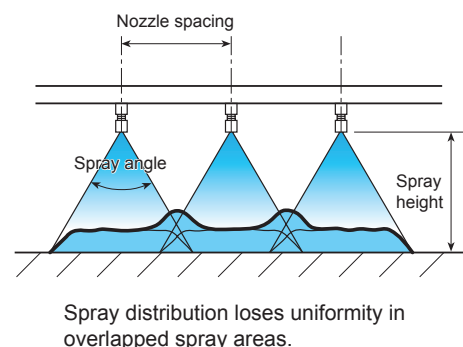
(C) Multi-nozzle arrangement using even flat spray nozzles
