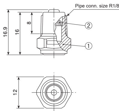
① Nozzle body ② Whirler
