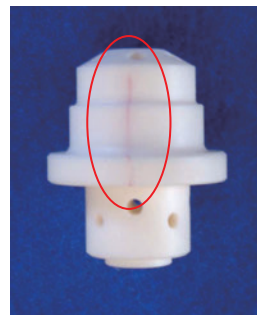
Nozzle cracked due to abrupt cooling
