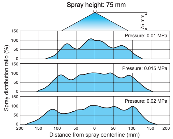
Relation between spray pressure and spray distribution
