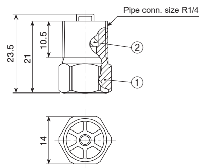
① Nozzle body ② Whirler
