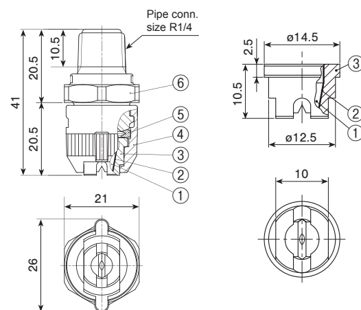
Nozzle Tip (① + ② + ③)
