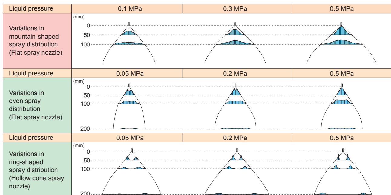
Ring-shaped distribution
